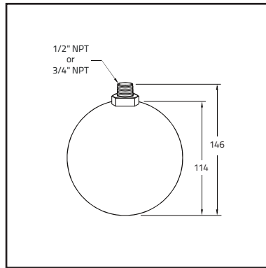
Ball Float
