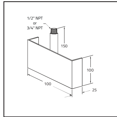
Extension Plate
