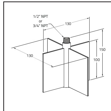
Cross Paddle
