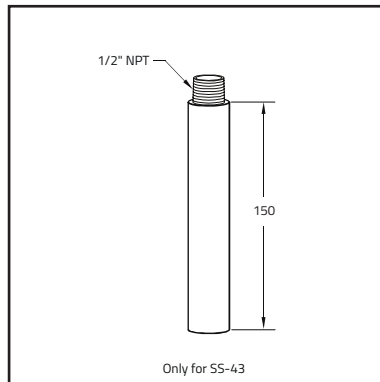
Wear Probe
